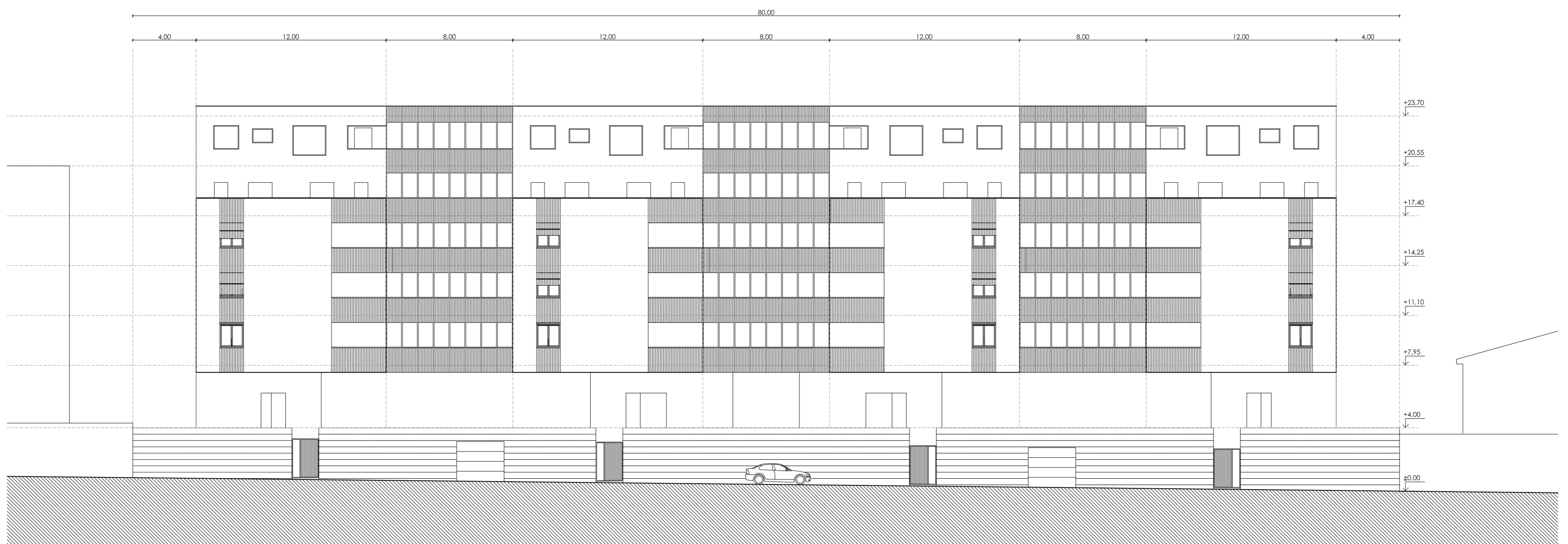
ALZADO PRINCIPAL
